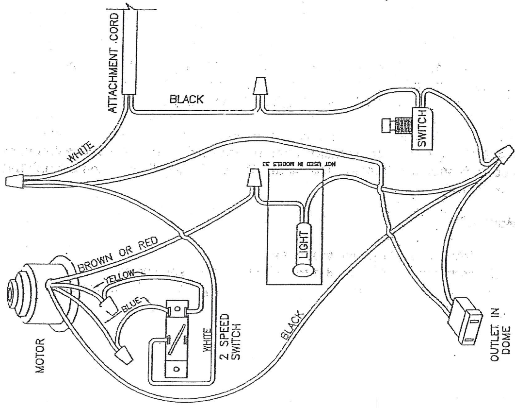
NEW MOTOR 5008001100
