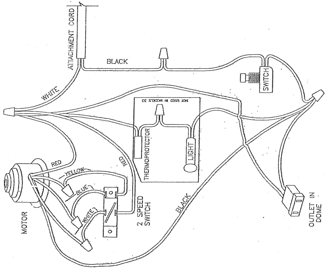
OLD MOTOR 5008001000
